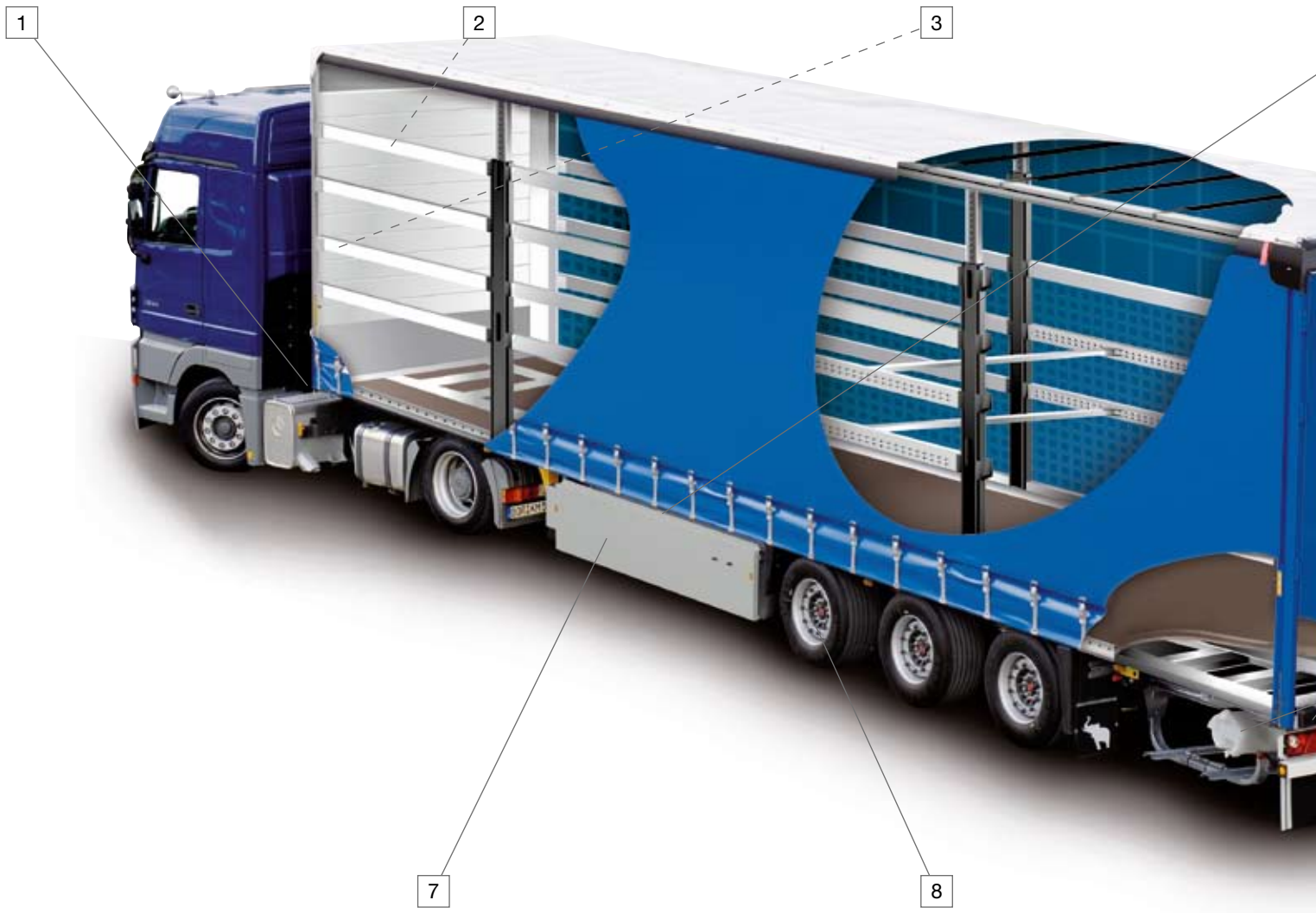
1 Front release device for quick opening and closing of the side tarpaulins
