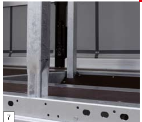
Four pairs of coil combi-supports for the body (80 x 80) and outer frame (70 x 70) according to SIDMAR regulation
